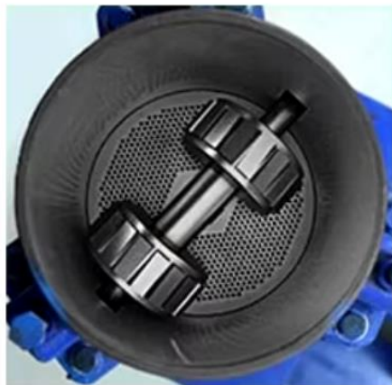
Two roll
