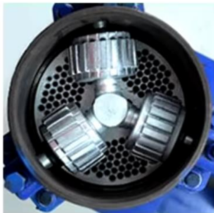
Three roll
